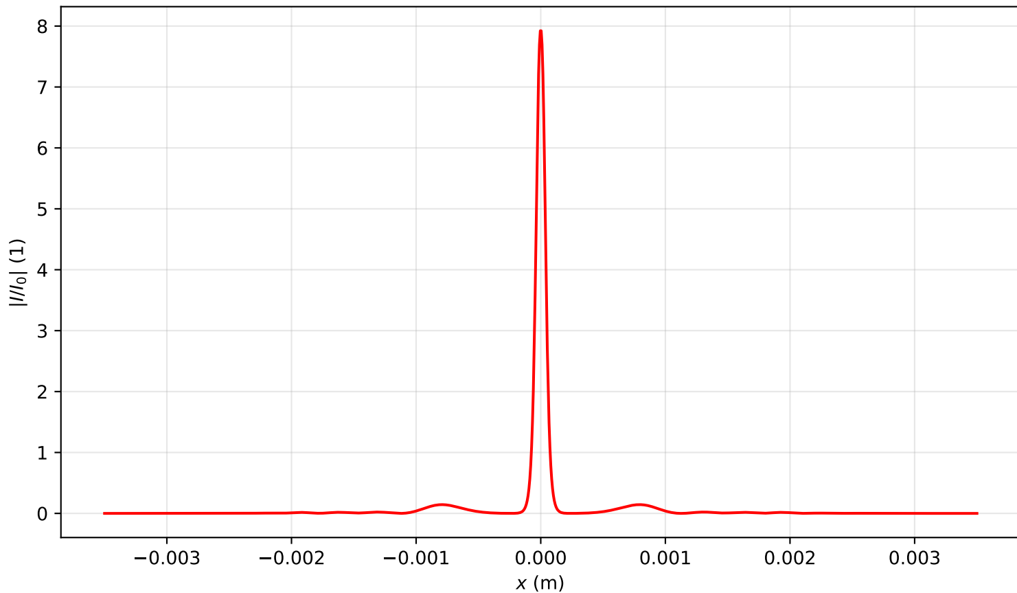
Intensity profile I(x, y = 0, z = 0.637)/I_0 , \text{Pin}=8.0\text{Pcr} , artificial time
